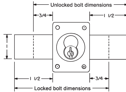
Long bolt option
